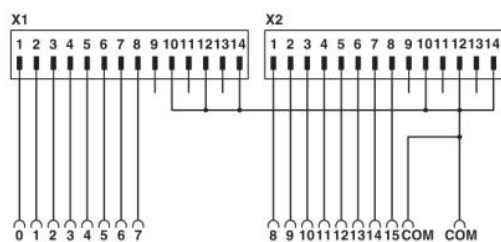
Connection scheme FLKM 14-PA-SLC500/IN
